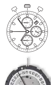
6S21 Height 4.50mm Chrono min / sec, 120 second 4 year battery life (SR927W)
