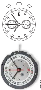
6S30 Height 4.50mm Chrono min / sec, 120 second 4 year battery life (SR927W)
