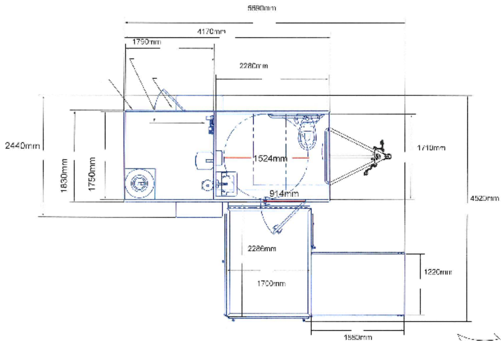
PLANM01: General Layout
