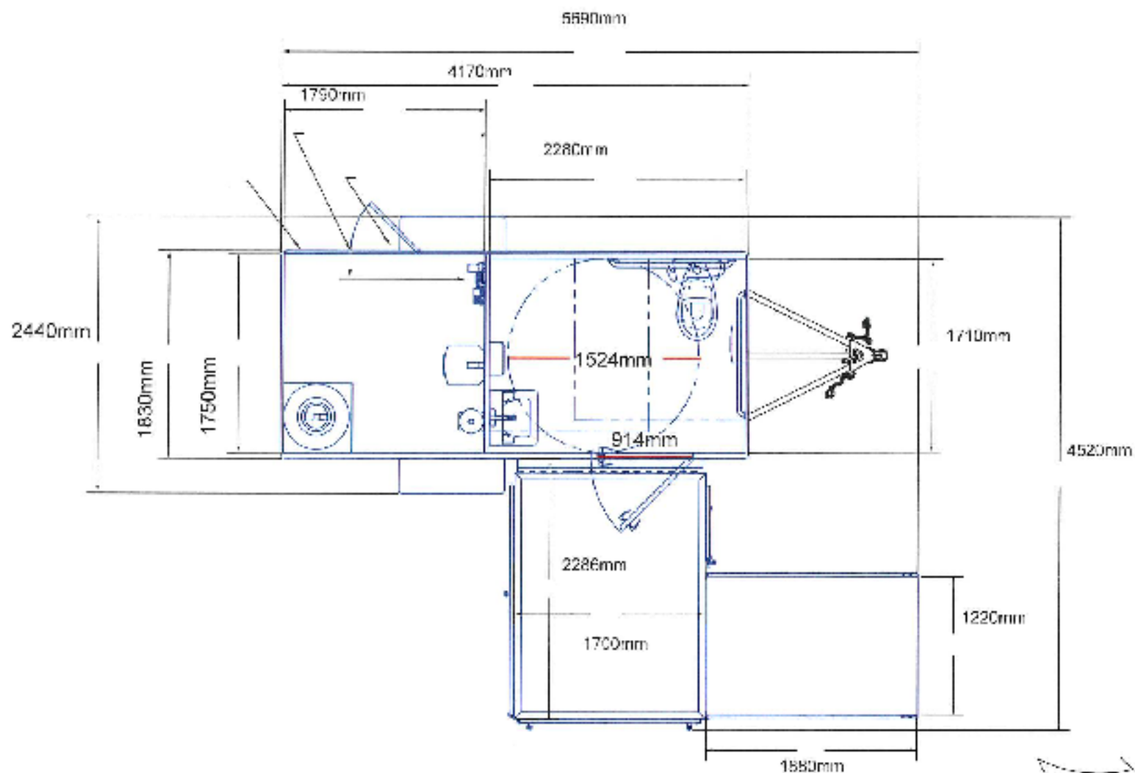
PLANMCH: General Layout
